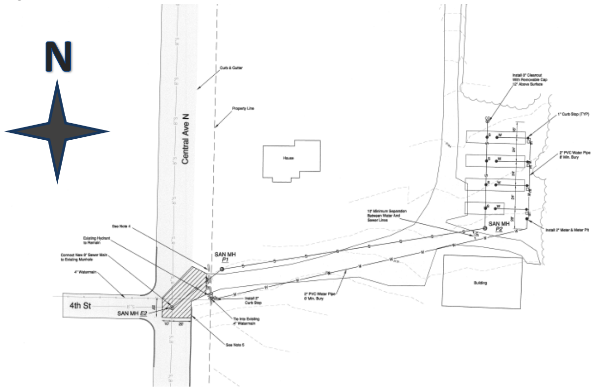
Figure 2. Preliminary Layout of Proposed Temporary Housing Units Marathon Oil Company – Zoning Map Change Application August 3, 2012
